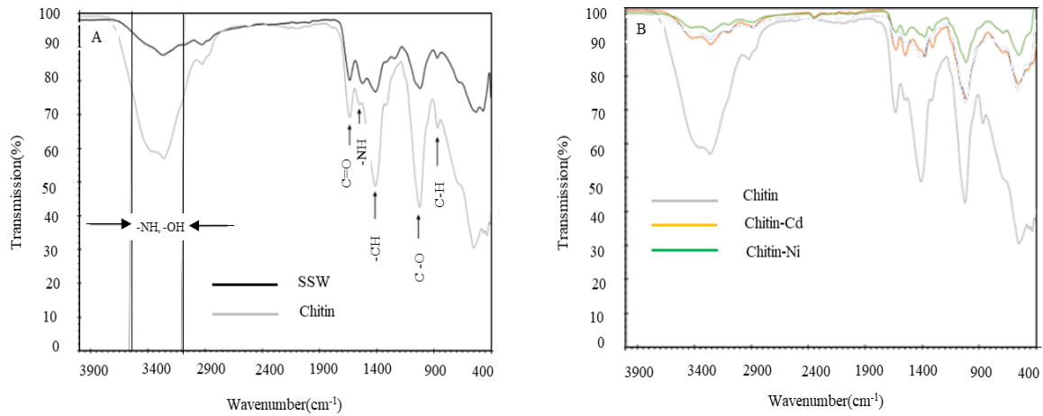
Figure 2. FT-IR analysis on (A) SSW and chitin; (B) chitin and chitin loaded with Cd(II) and Ni(II)
