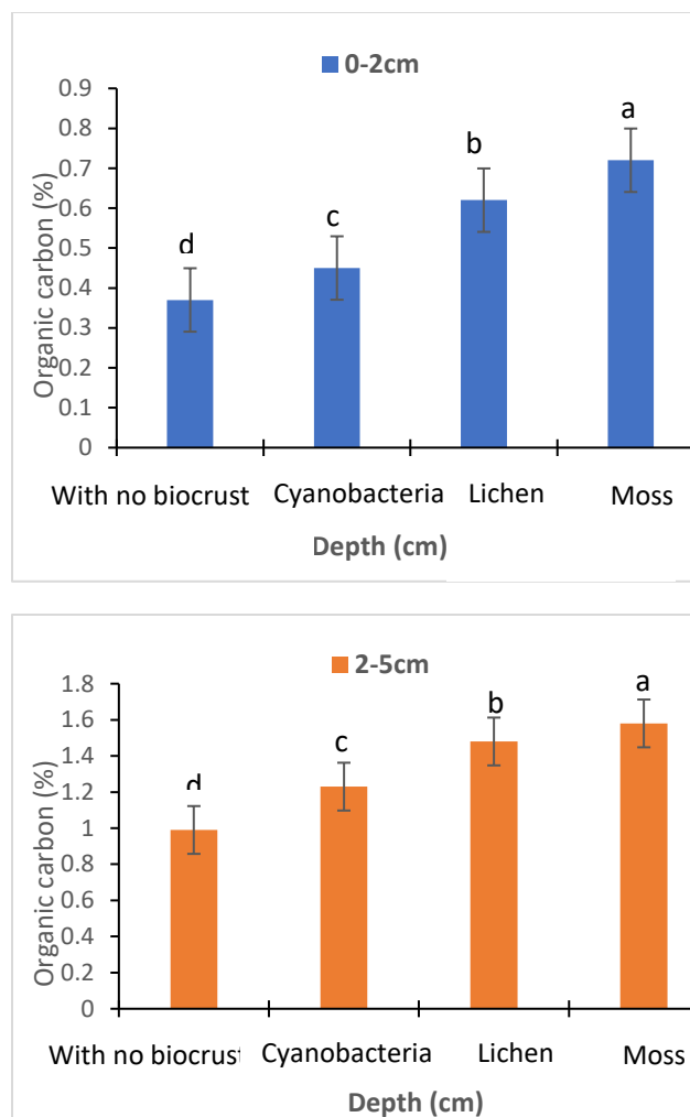
Fig.2. The effect of biological crusts and no crust on subsoil organic carbon at two depths (0-2 and 2-5cm).
