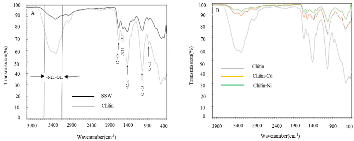
Figure 2. FT-IR analysis on (A) SSW and chitin; (B) chitin and chitinn loaded with Cd(II) and Ni(II)
