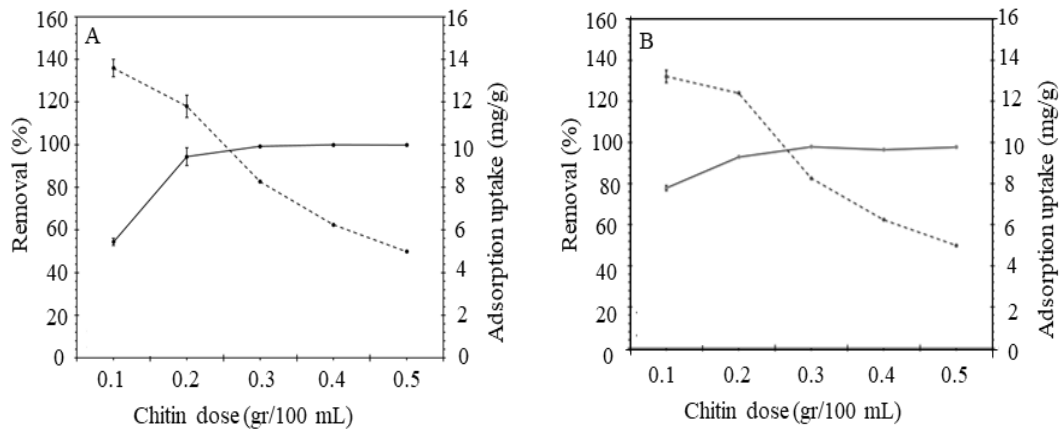
Figure 3. Effect of chitin dosage on removal and adsorption uptake: (A) Cd; (B) Ni
