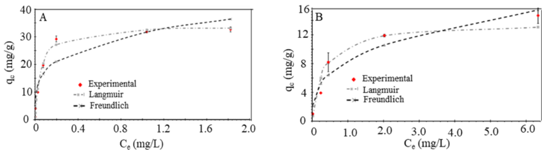
Figure 4 Langmuir and Freundlich isotherm models of the adsorption for A: Cd and B: Ni on chitin
