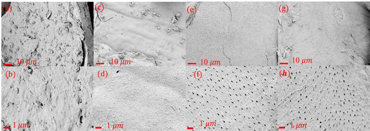
Figure 1. SEM analysis (a) and (b) original SSW; (c) and (d) chitin (before adsorption process); (e) and (f) chitin loaded with Ni(II); (g) and (h) chitin loaded with Cd(II).
